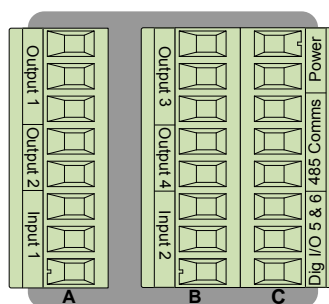
Back View Slot Orientation 1/16 DIN PM6
