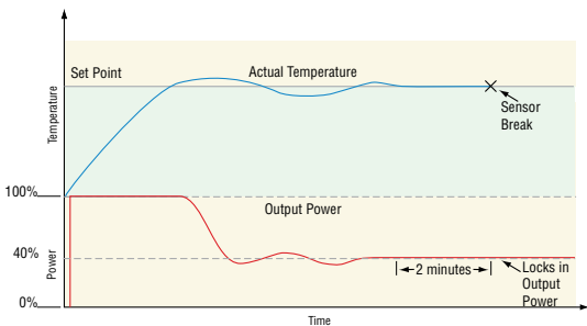
Bumpless Transfer
